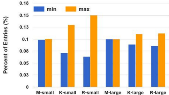
Figure 11: Load balancing efficiency of different hashing methods. M, K and R stand for Maglev, Karger and Rendezvous, respectively. Lookup table size is 65537 for small and 655373 for large .
